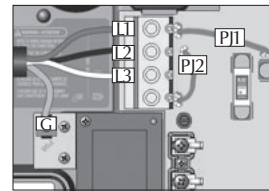
2-phase used from 3-phase Delta – no neutral Use 2-phase setting L1+L2 currents return through L3 Connect P1 between P7 and P10. Connect P2 between P13 and P74.
