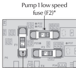
Pump 1 high speed fuse (F1)
