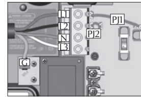
3-phase with single neutral L1, L2+L3 currents return through neutral Connect P1 between P7 and P10. Connect P2 between P11 and P13.
