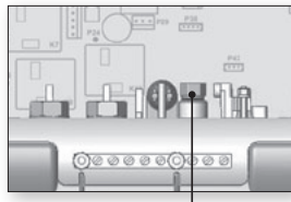
GFCI/RCD (J1)
